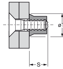
Full Collar
