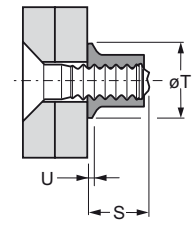
Flanged Collar
