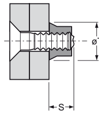
Half Collar
