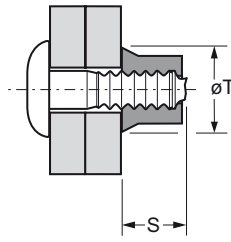
Full Collar
